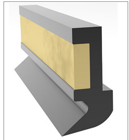
TSA-M19 WIPER W/ BRASS (Purchased as separate units)
